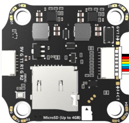
F7 V3 Flight Controller
